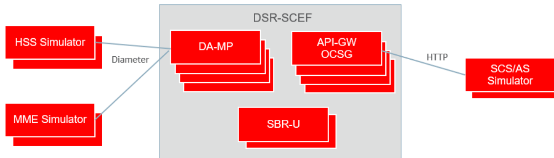
Figure 8: SCEF Testing Topology
