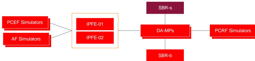
Figure 5: SBR Testing Topology
