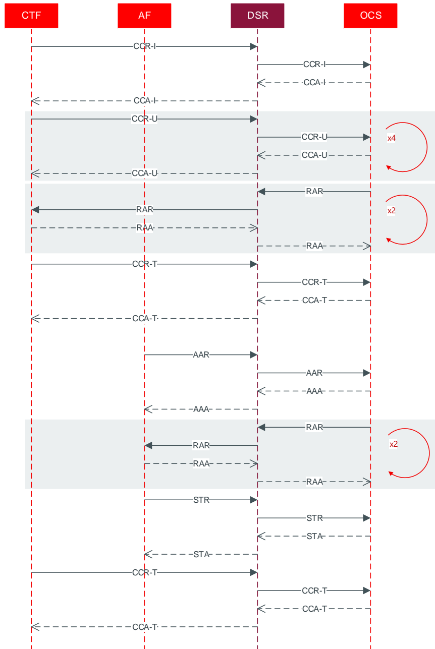
Figure 6: PDRA Message Sequence
