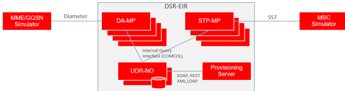
Figure 9: EIR Testing Topology
